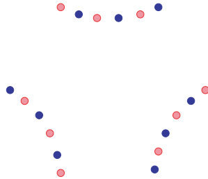
FIG. 1. Example without empty monochromatic 4-gons.
