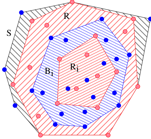
FIG. 2. Red and blue layers in the proof of Lemma 5.
