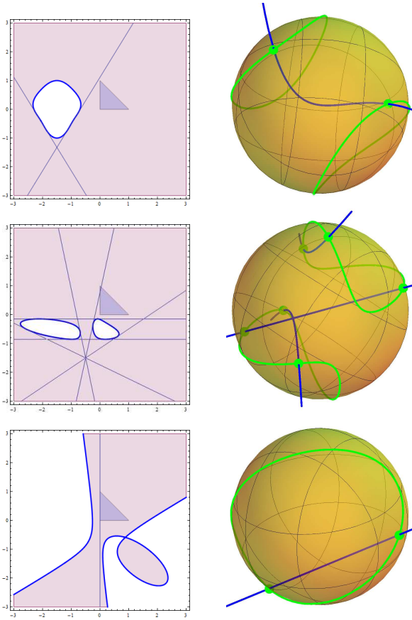
Figure 2: Left: Exceptional lines (thin blue), the curve C(u, v) = 0 (thick blue) and the domain triangle \Delta . Right: The curve \mathcal{S}_\Sigma (green), exceptional isotropic normals (green points) and the exceptional set \mathcal{E} (blue). Top row: Example 1, patch \mathbf{p}_1(u, v) ; Middle row: Example 1, patch \mathbf{p}_2(u, v) ; Bottom row: Example 1, patch \mathbf{p}_3(u, v) .
