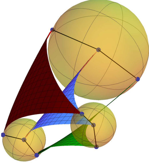
Figure 1: Bisector surface (blue) and two branches (red and green) of the envelope surface forming a boundary of a volume V .
