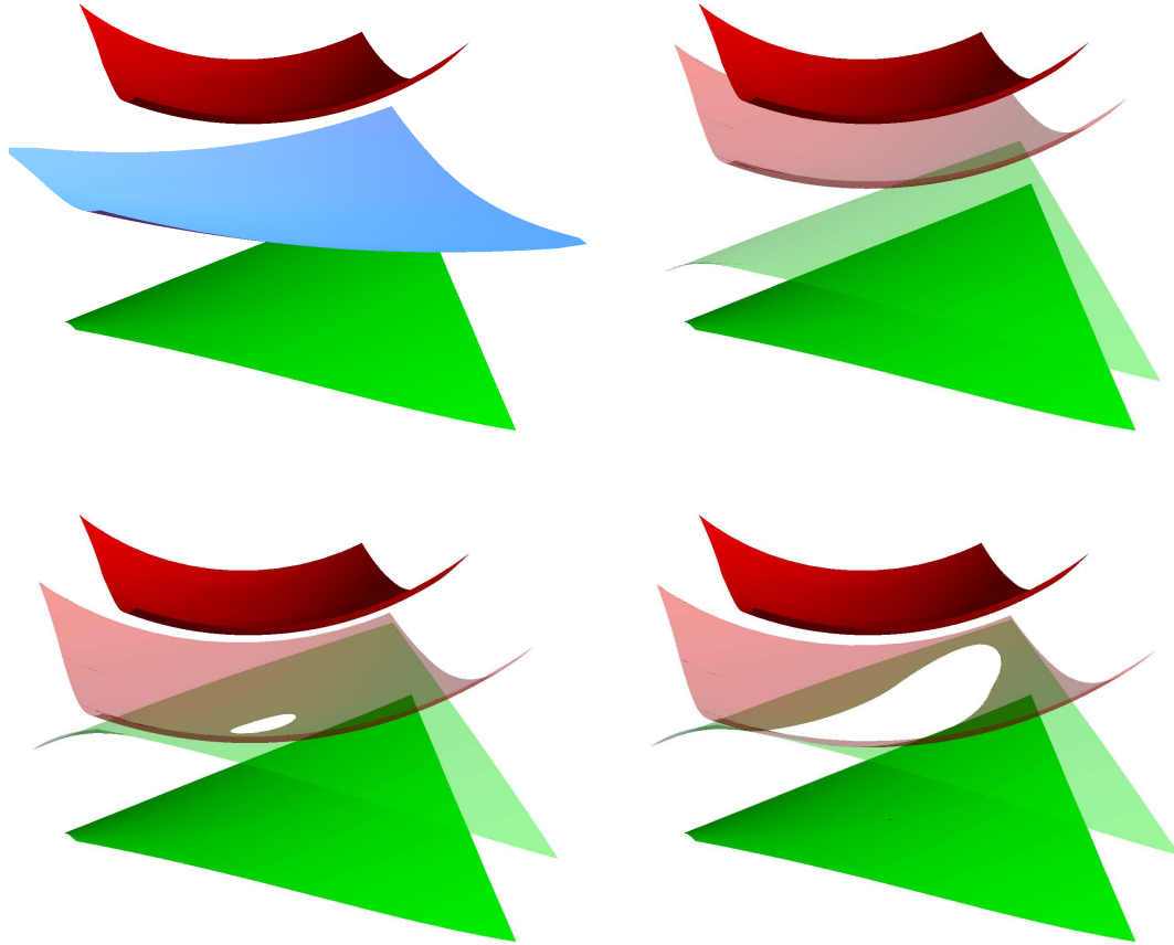
Figure 7: Bisector surface (blue) and the two branches of the envelope (red and green) in Example 2, along with the trimmed inner offsets (light red and light green) – without self-intersection (top right) and with self-intersection (bottom left and right).
