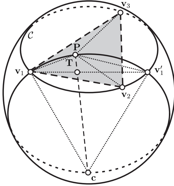
Fig. 2. The points used for the geometric proof.
