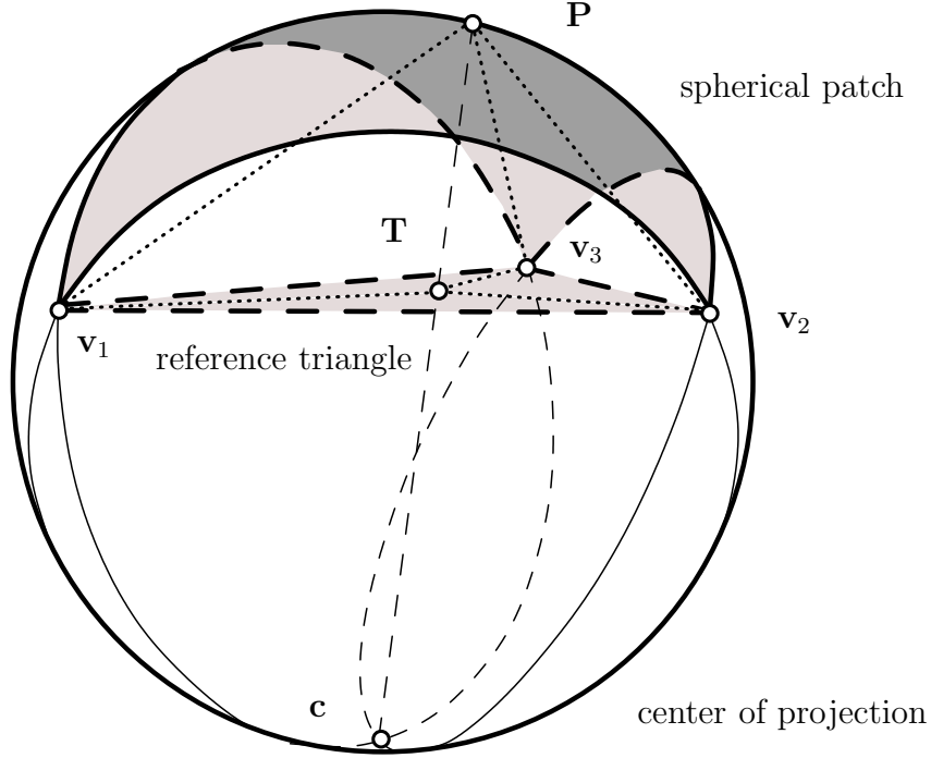
Fig. 1. A quadratic triangular patch on the sphere with the reference triangle \Delta(\mathbf{v}_1, \mathbf{v}_2, \mathbf{v}_3) and the center of projection \mathbf{c} .
