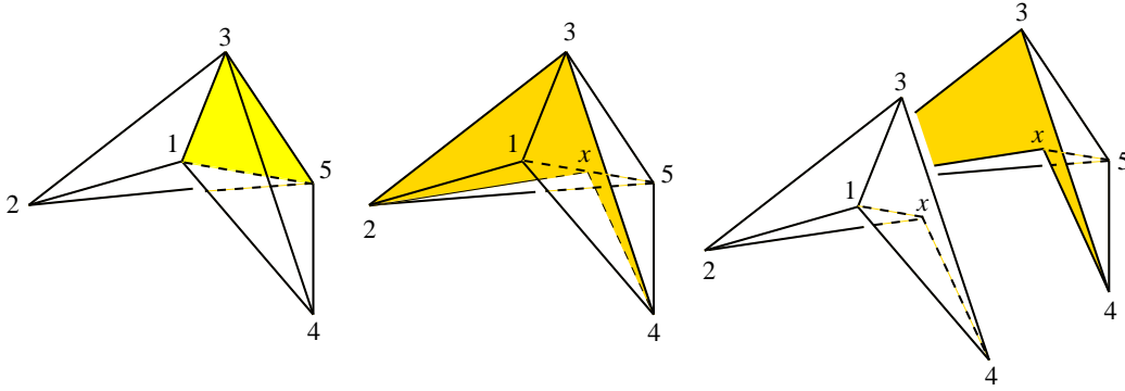
Figure 5: Exchanging pseudoflip
