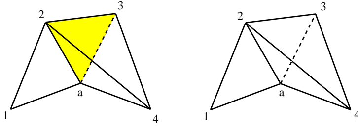
Figure 4: Removing pseudoflip
