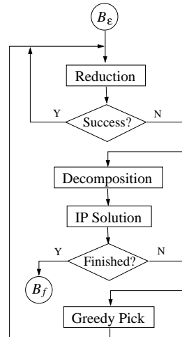
Figure 2: Control flow of the algorithm
